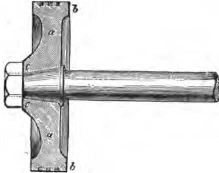
FIG. 235.—The Piston of a small double-acting steam engine, showing method of connecting the piston rod, and the position of the packing rings. The parts are: a, a , the body of the piston; b, b , the circumference bearing the packing rings; c, c , the central boss receiving the coned end of the rod.
